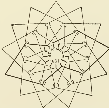
Fig. 137. Diagram Showing the Effect of Short-Circuit Between Two Coils
